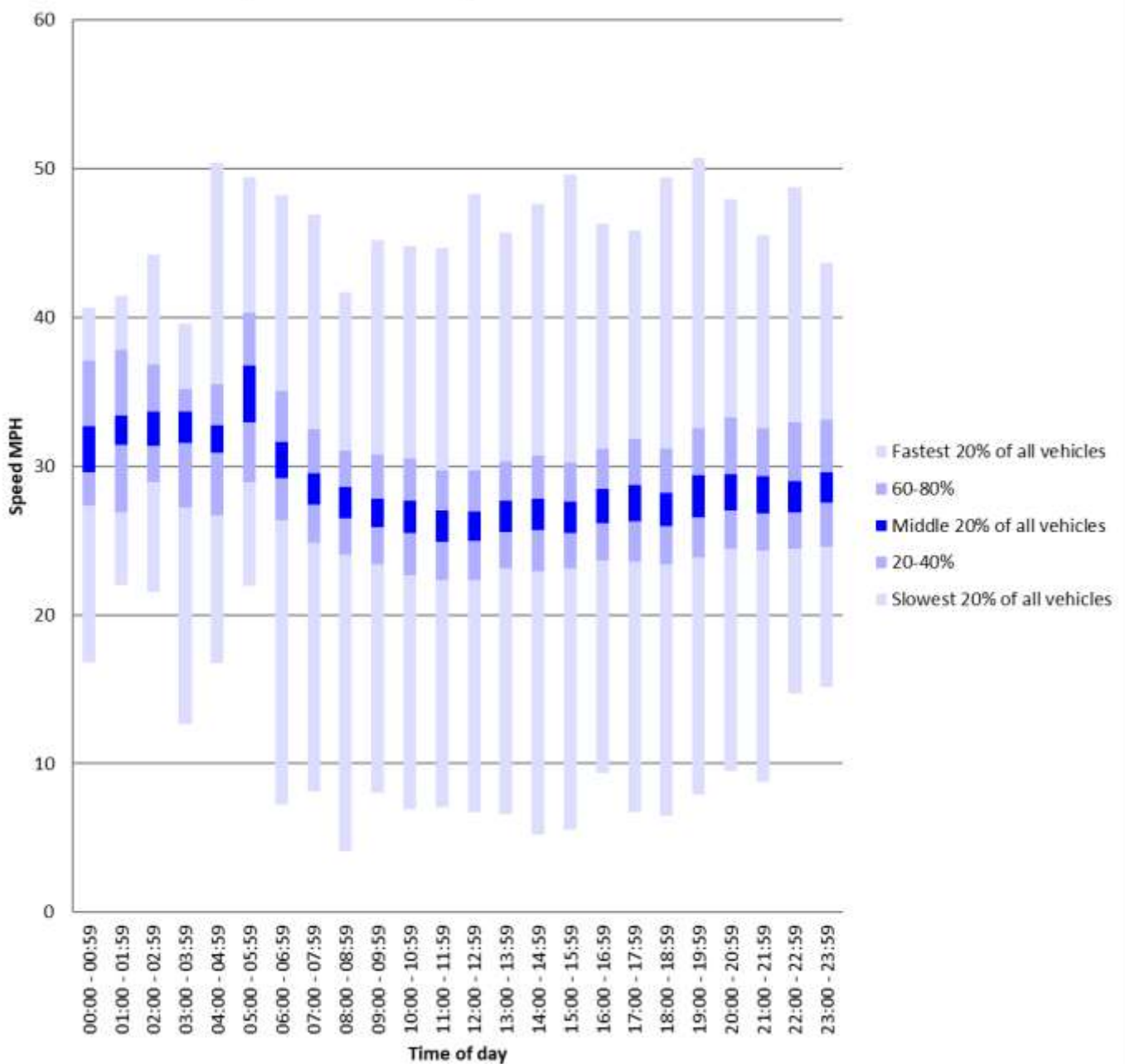
Speed Summary - Teeton Road March 2020
